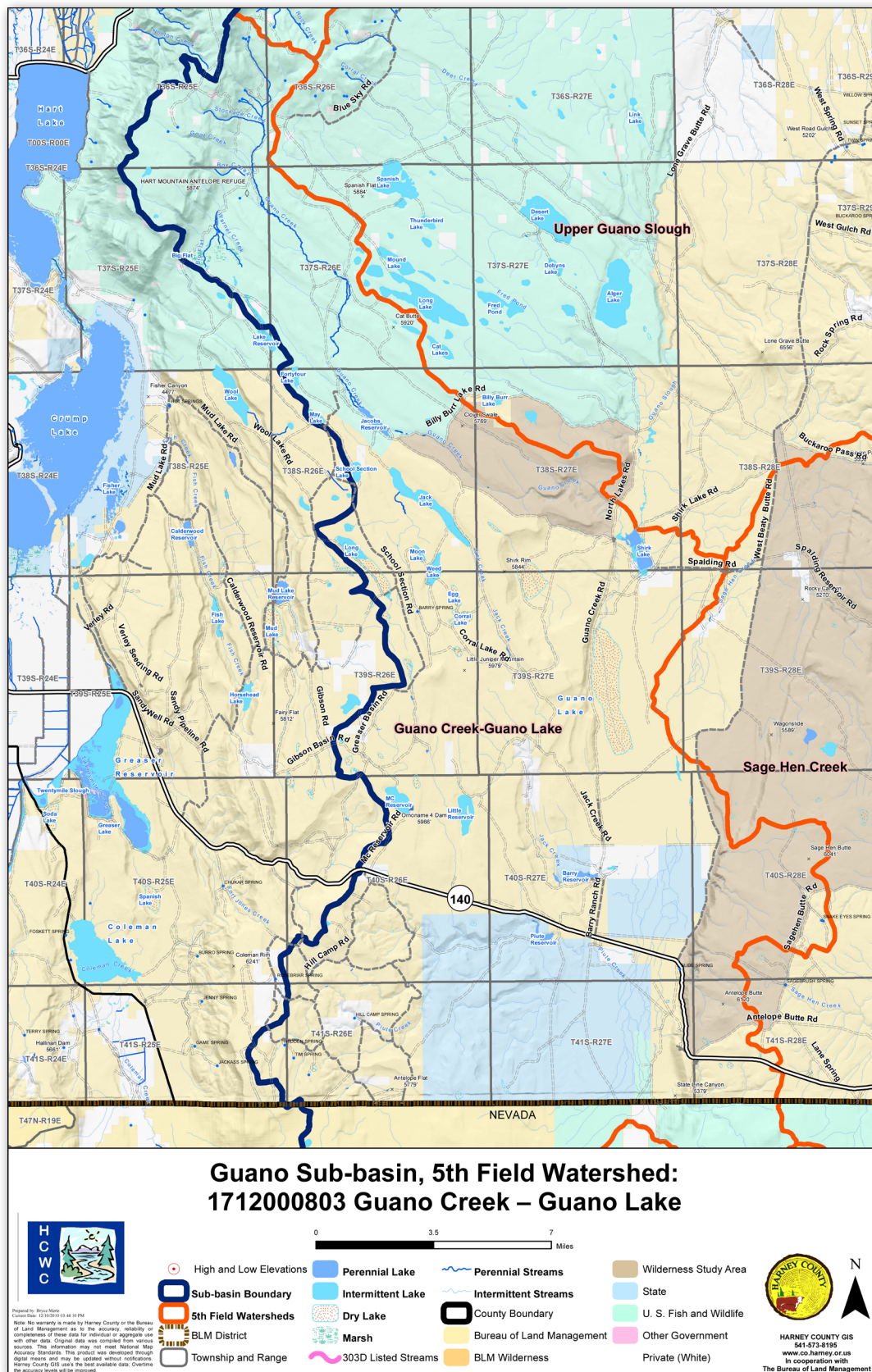
Map 3-8. Guano Creek - Guano Lake watershed.
