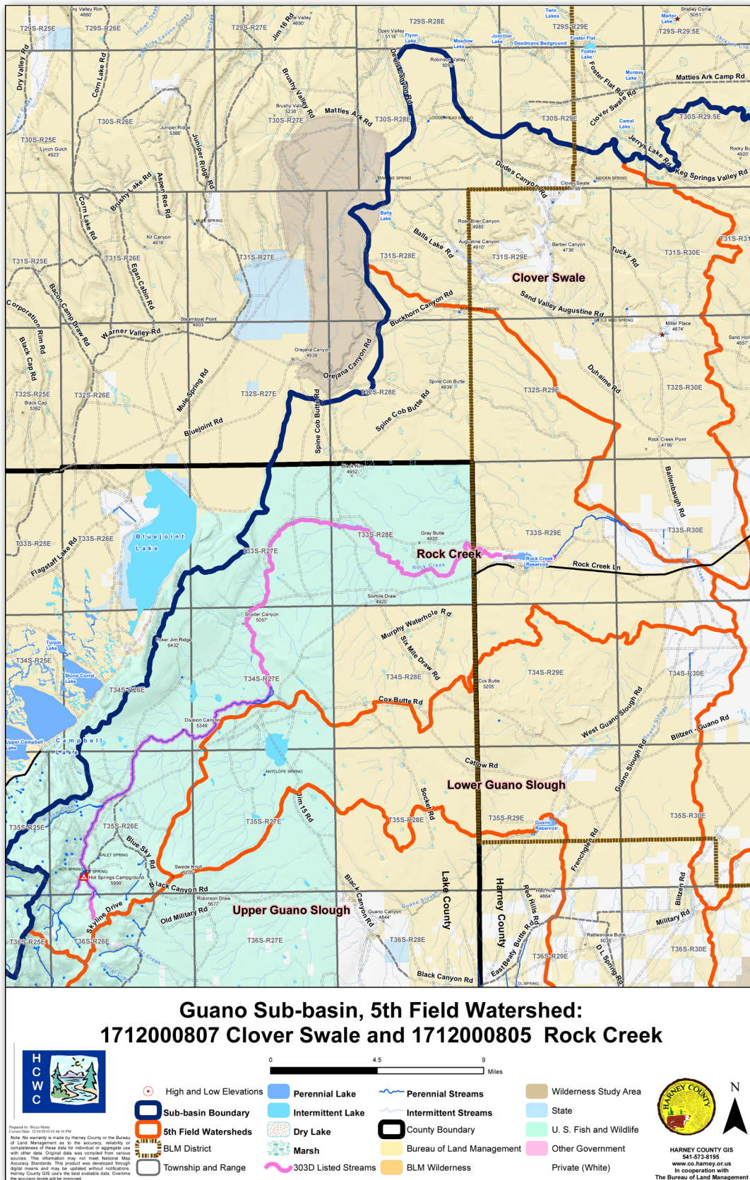
Map 3-7. Clover Swale and Rock Creek watersheds.
