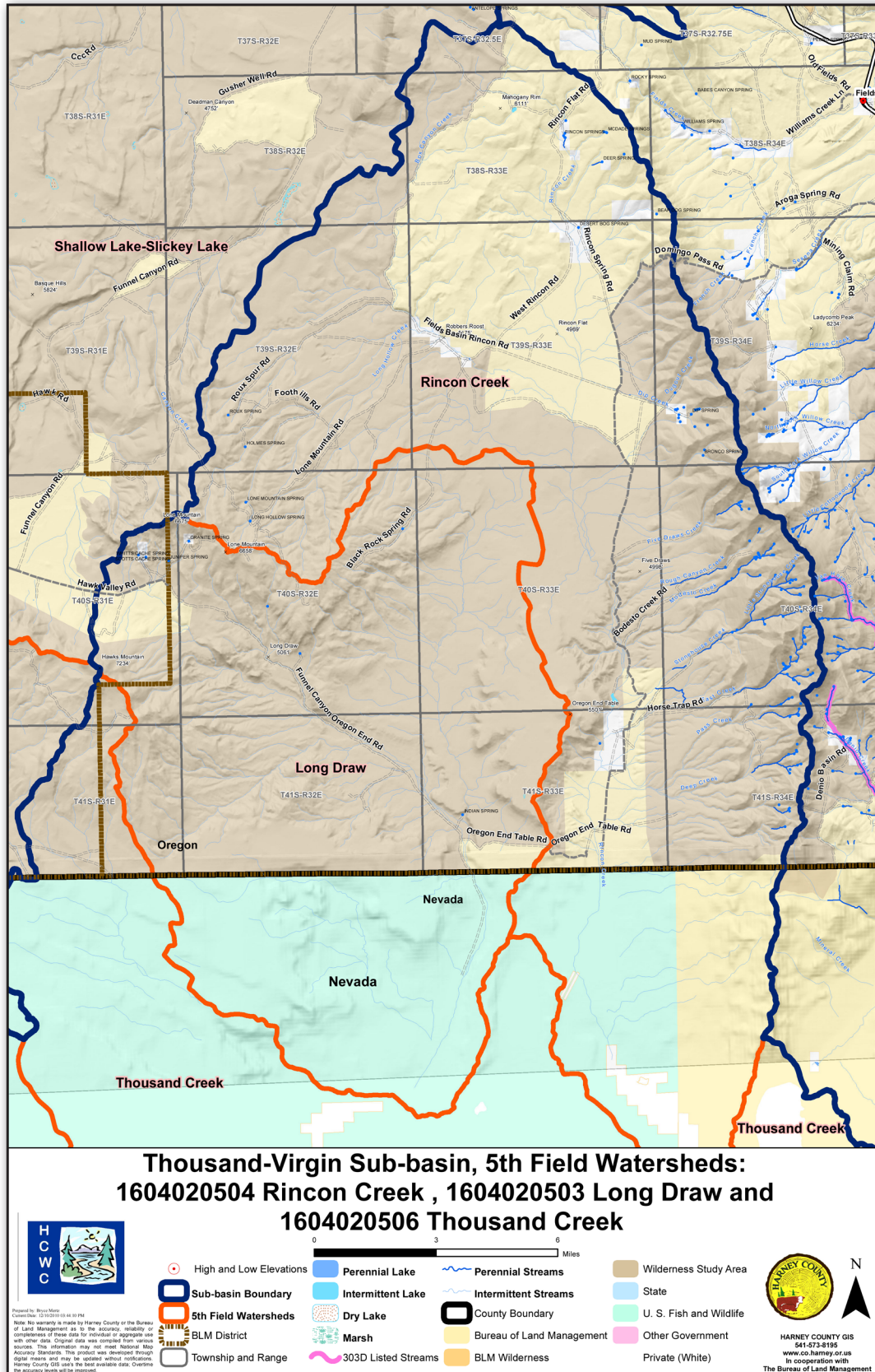
Map 3-6. Rincon Creek, Long Draw, and Thousand Creek watersheds.
